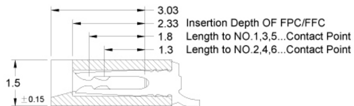
SECT X-X'
