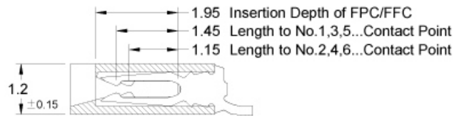
SECT X-X'
